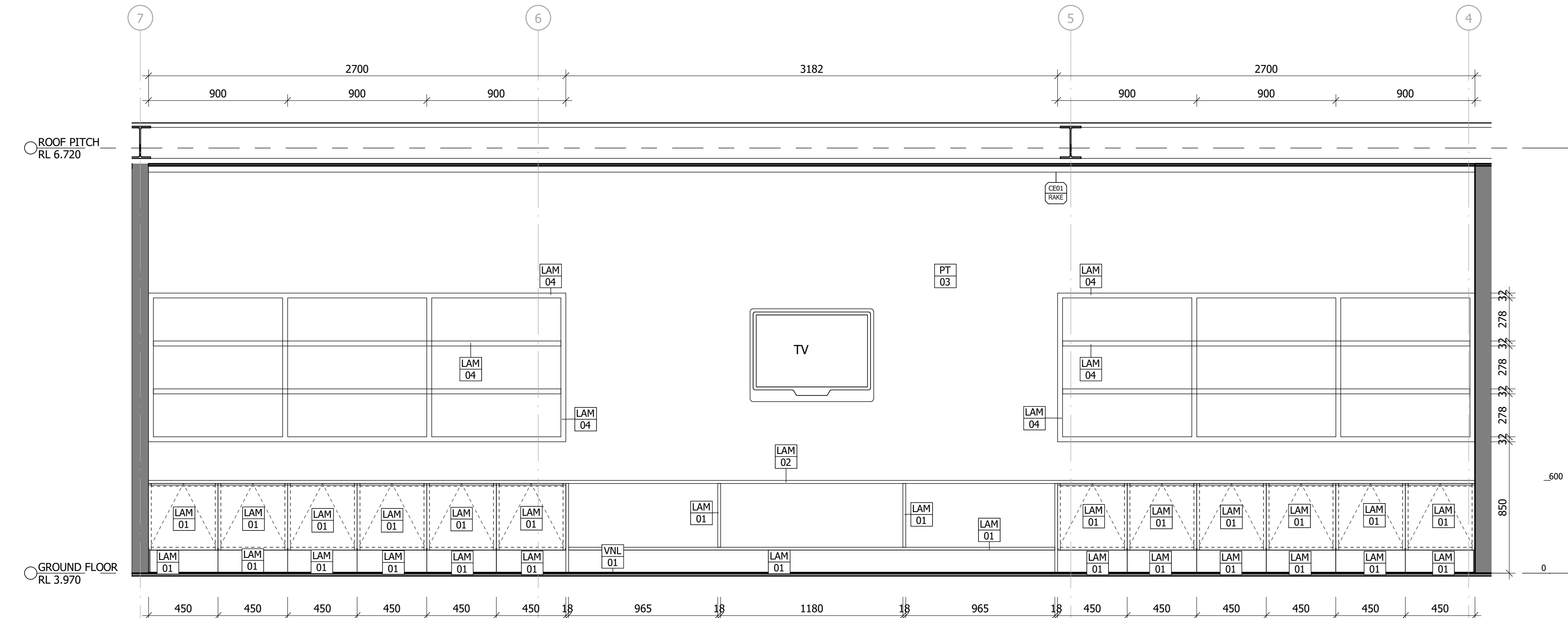
2 J02 - ELEVATION 1 - RECREATION A4501 1 : 20
